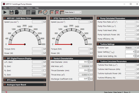
TYPICAL SCREENSHOT OF THE OPTIONAL VDas® SOFTWARE
